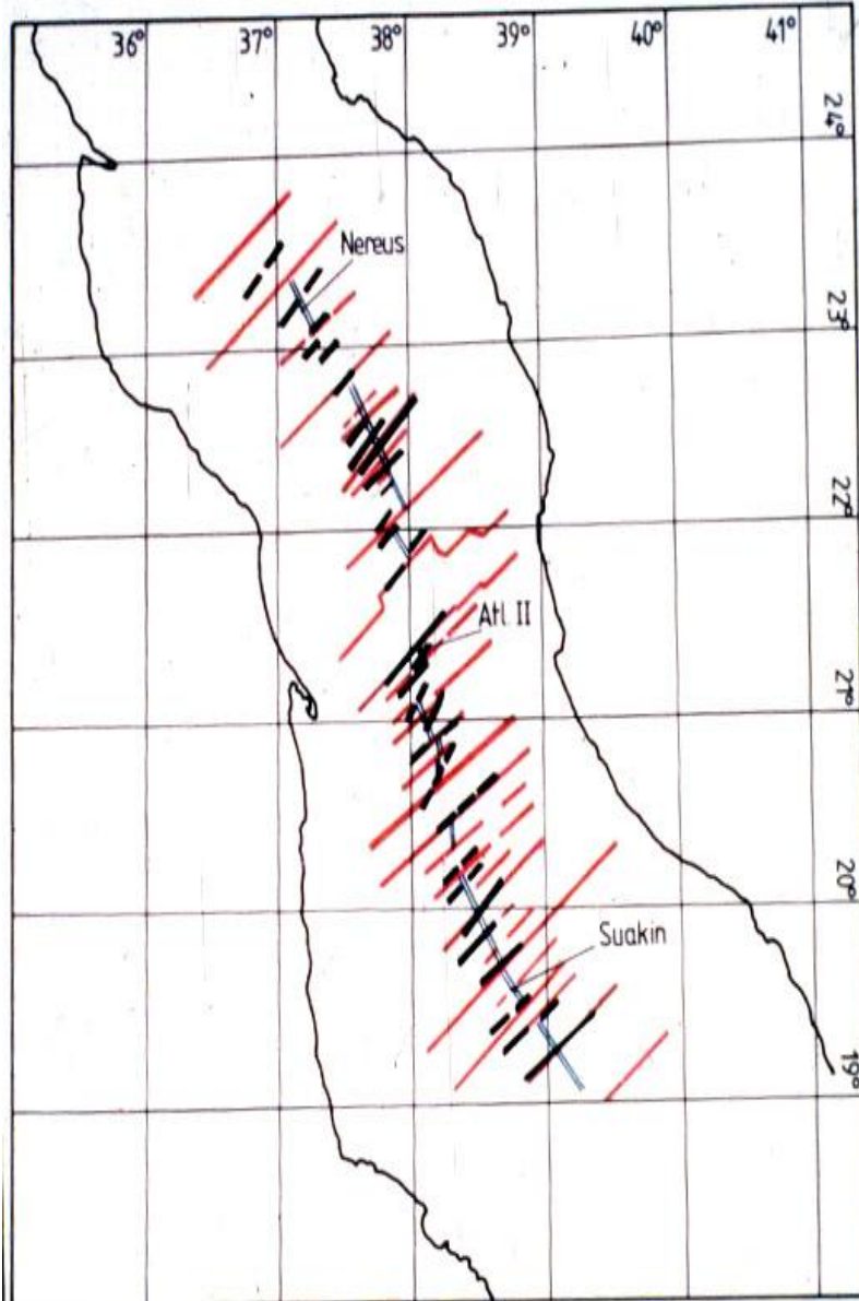
Presumed location of transform faults in the central Red Sea
